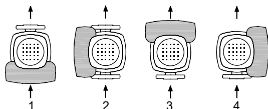
Terminal box positions
